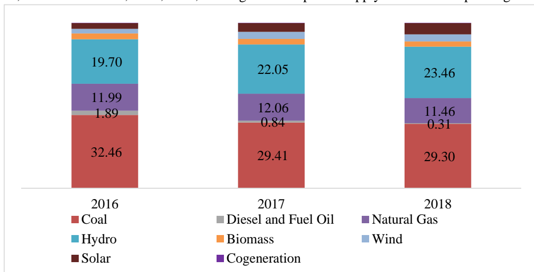
Figure 3. Electric power generated by power plants in SEN grid by fuel type (TWh, 2016-2018) (Note: the figure is developed based on National Energy Commission (2020).)
